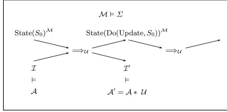
Fig. 2. Fluent Calculus semantics for ABox-Update
